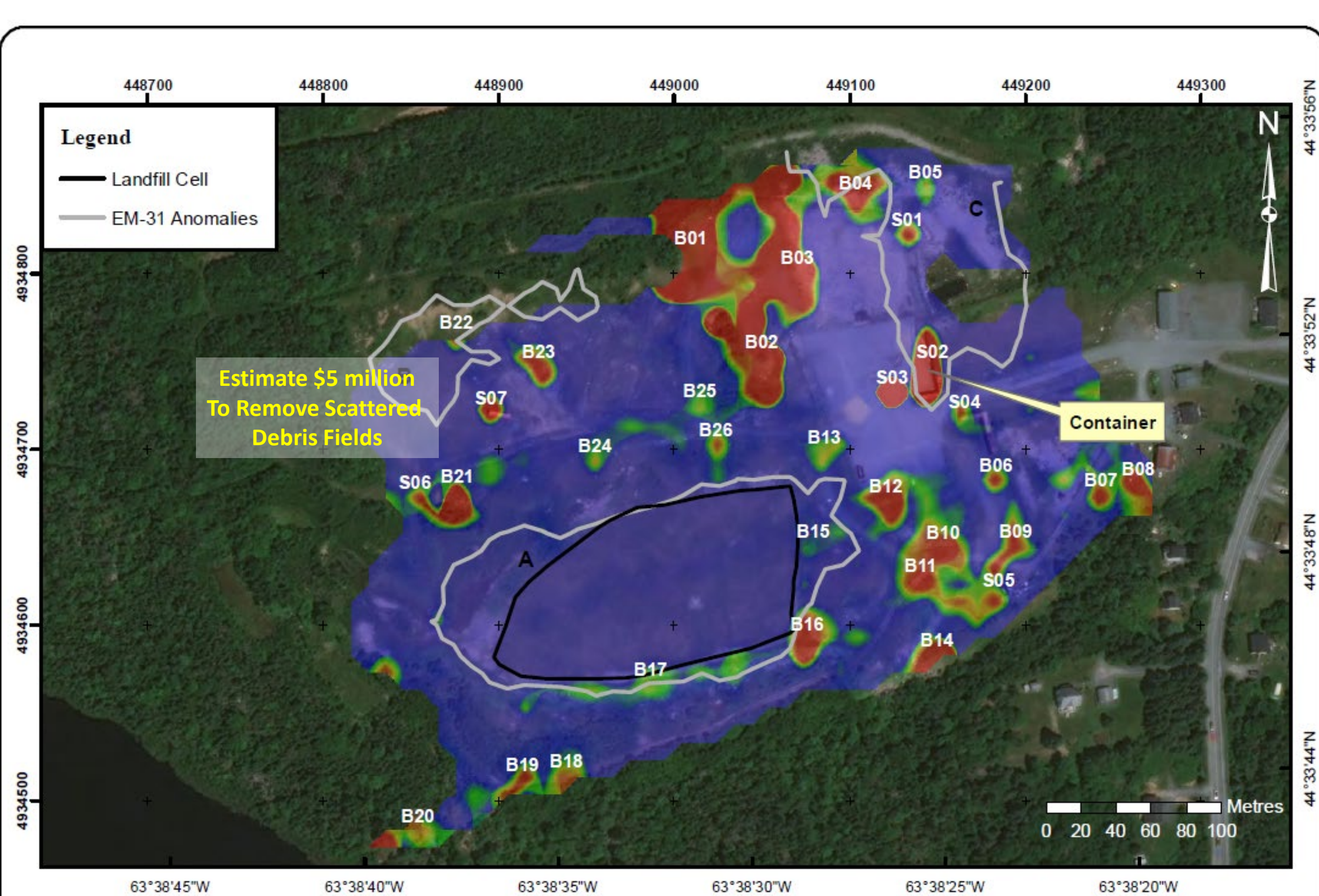
Figure 4.4.1: Shaded EM-61 anomaly map overlain with polygons outlining EM-31 conductivity anomalies.
