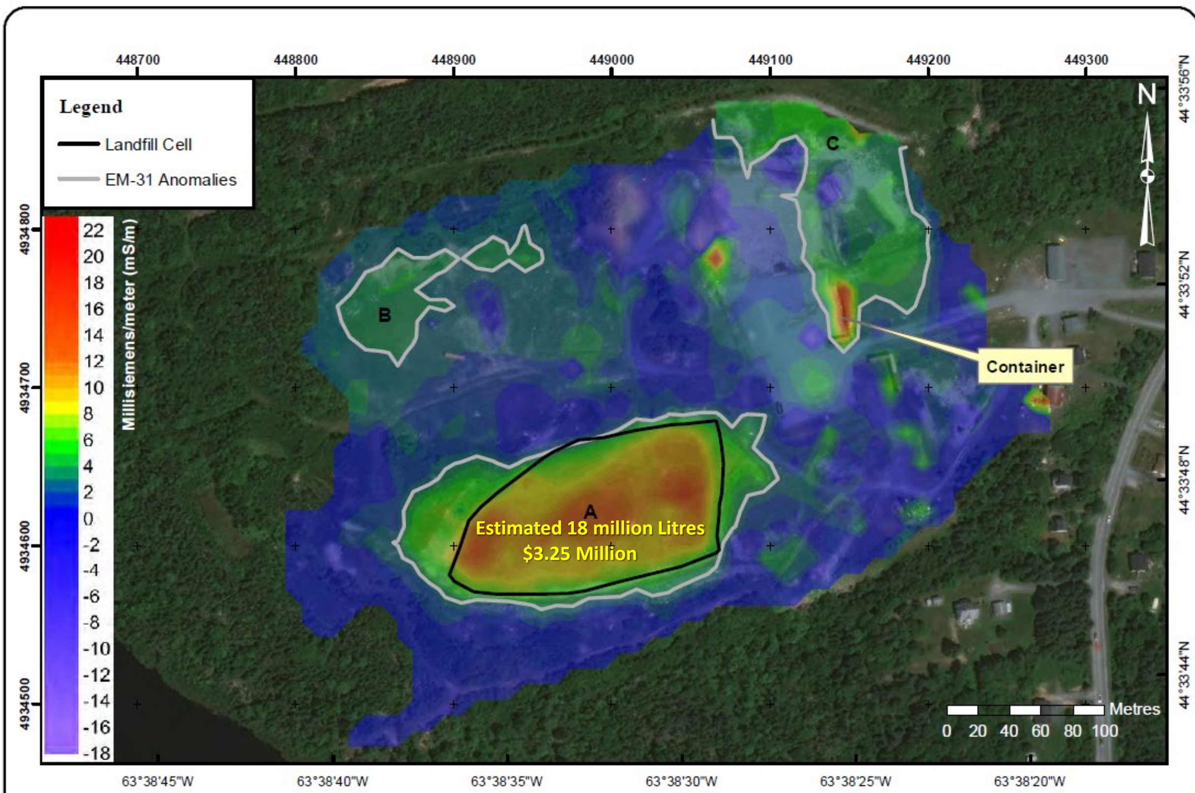
Figure 4.2.1: Vertical quad phase conductivity measured by the EM-31.
